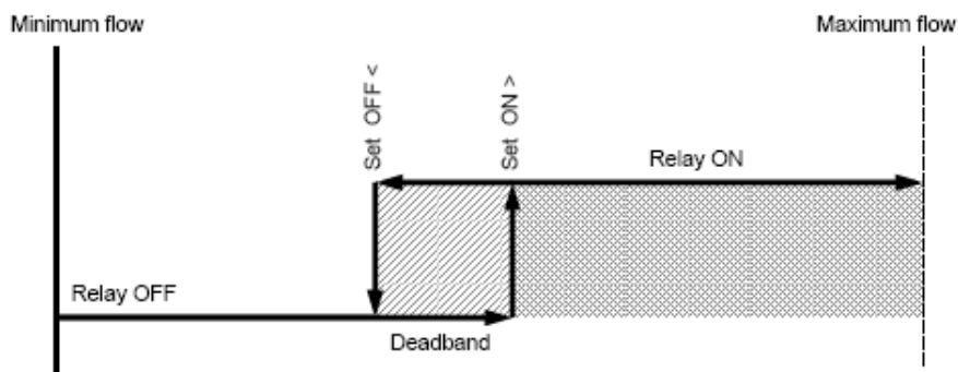
Fig 4.2 Single Point Alarm Operation
