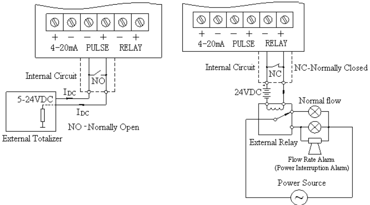
Fig 2.4A Passive Source Pulse Output
