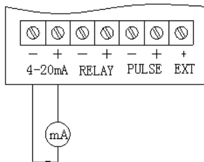
Fig 2.3 4-20mA
